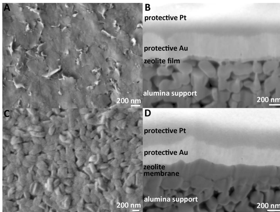
Figure 8. SEM images of the MFI-nanosheet films and their cross section prepared by FIB.
